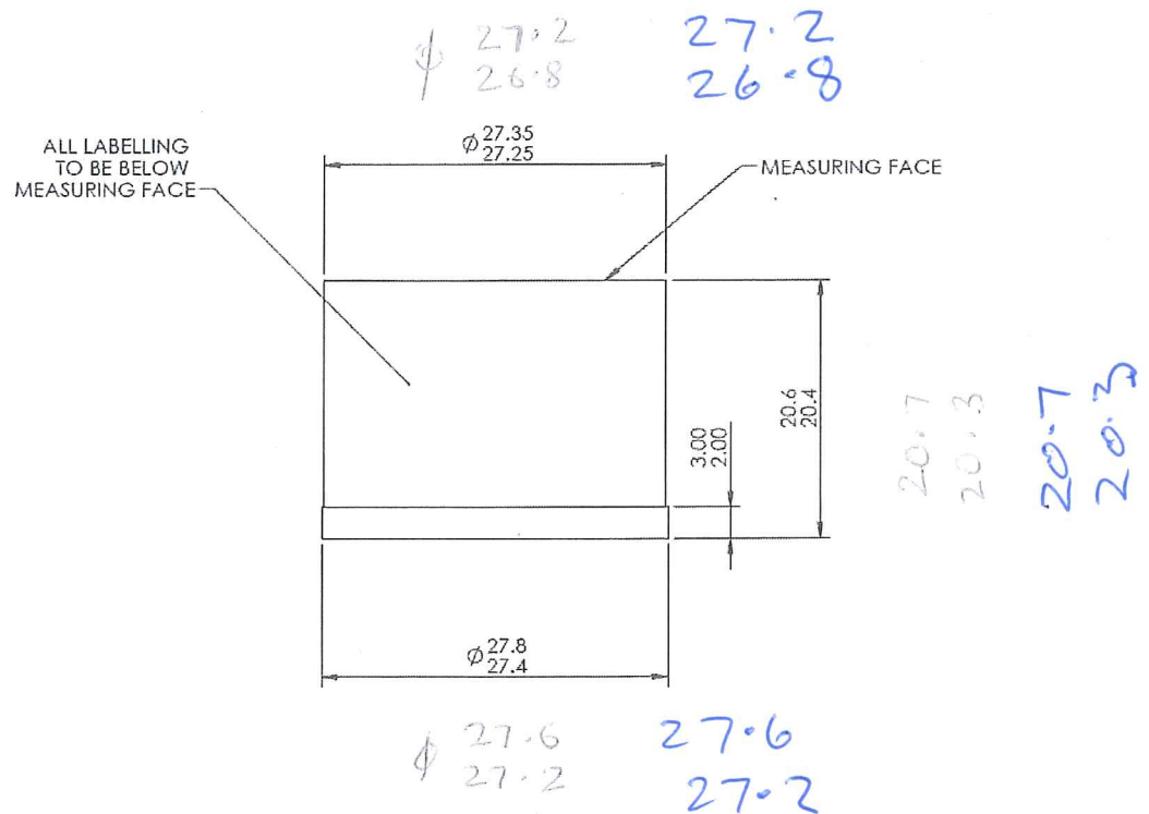
Figure 1 – Sensor Dimensions
