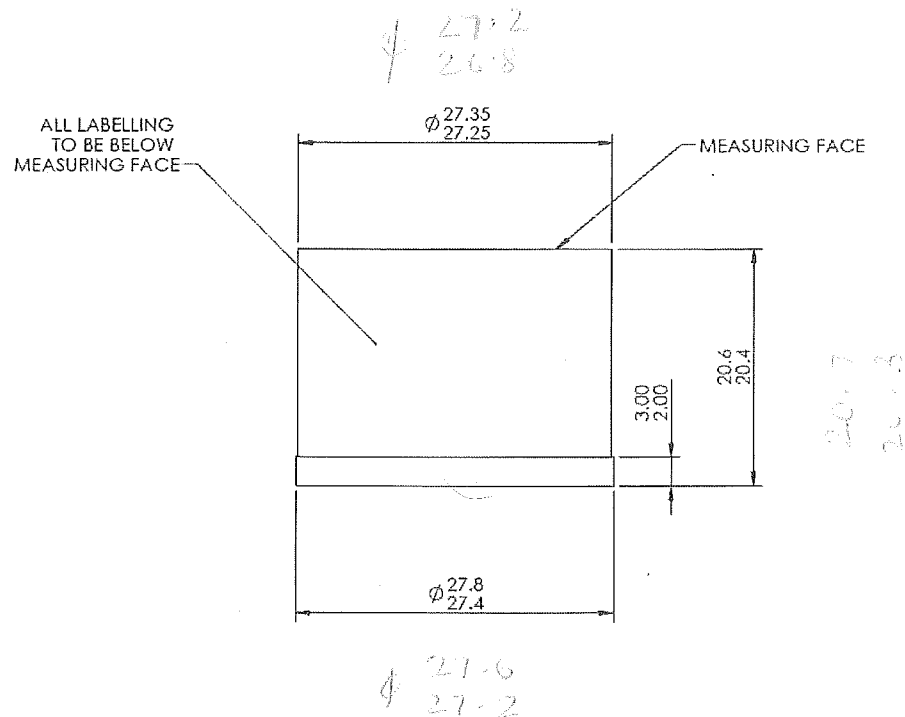
Figure 1 – Sensor Dimensions
