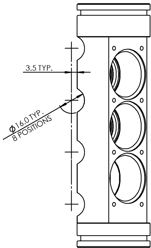
VIEW ON 'E'
