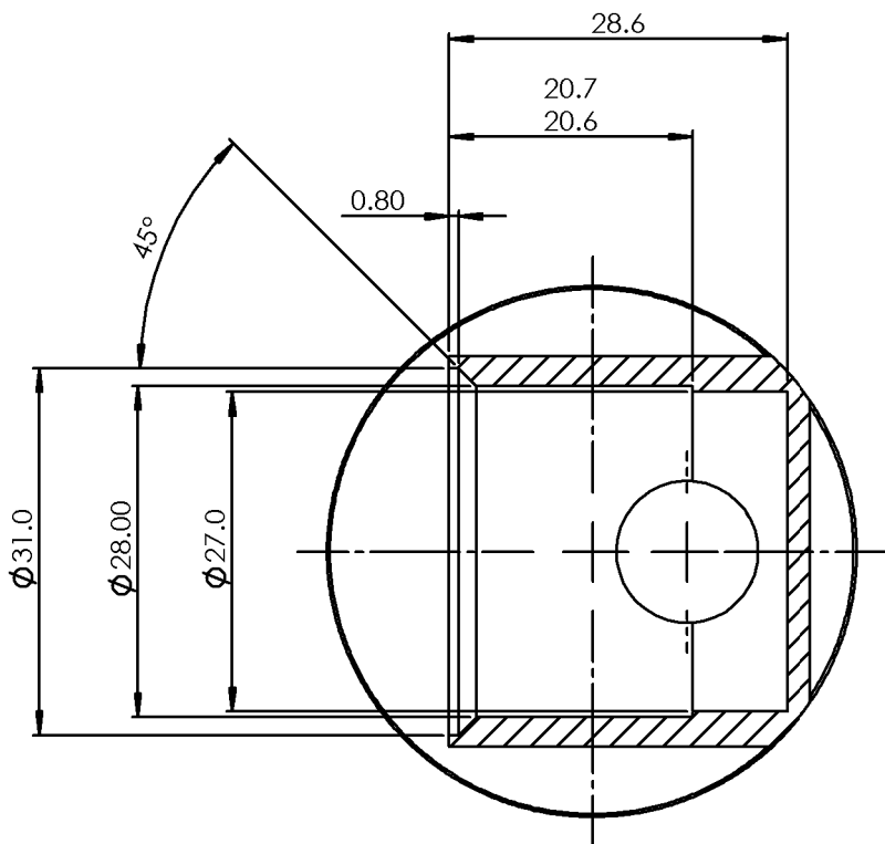
SECTION C - C (SCALE 2 : 1)
