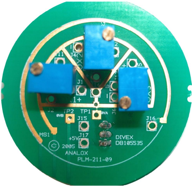
FACE VIEW
