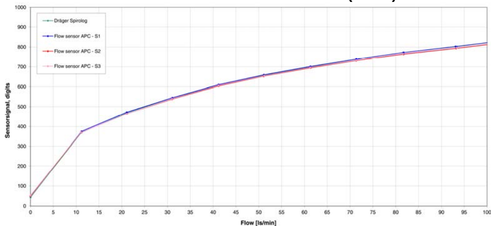
Statistical values before sterilization (134°C)
