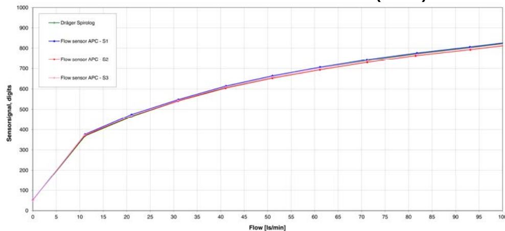
Statistical values after 100x sterilization (134°C)
