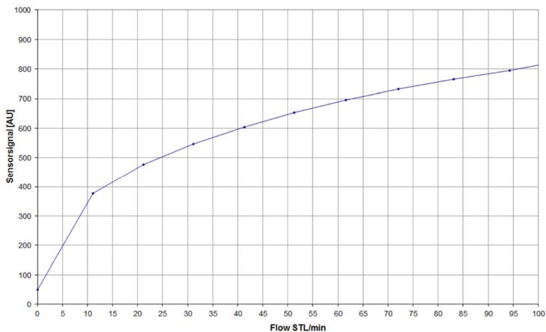
SpiroTrue A(PC) – typical flow curve with Flow-A module
