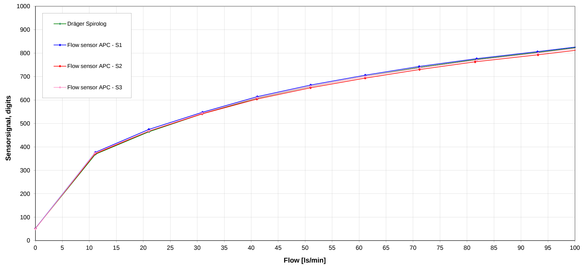
Flow sensor APC- statistically values after 100x sterilization (134°C)
