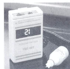
TED 60T Portable Oxygen Analyzer. Also available with 3rd Digit
