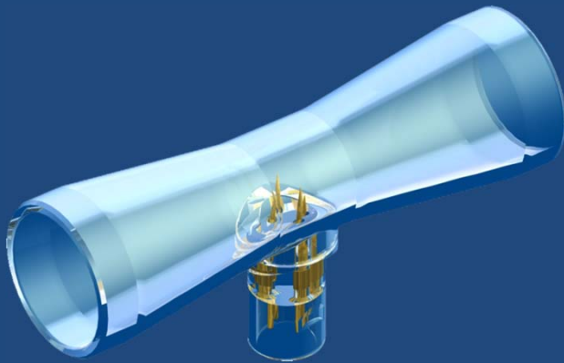
SpiroTrue A(PC) Hot-wire anemometric flow sensor for use with Dräger ventilators
