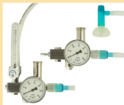
TT490 and TT480 Tom Thumb with NeoPEEP resuscitation circuit and mask
