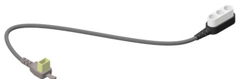
REF Part No. Description 5750108 2510102 Main Patient Cable* Overall assembly length: 262.5 cm, cable length 250cm
