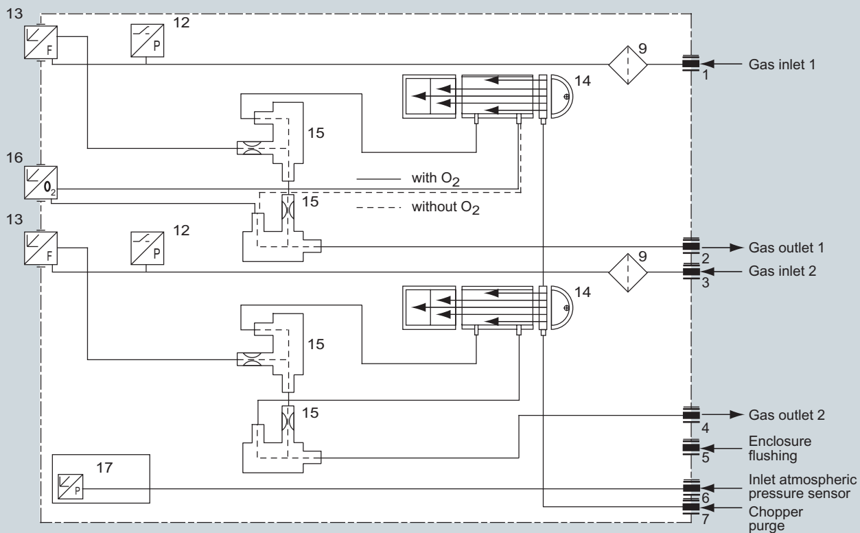
ULTRAMAT 23, 19" rack unit without internal sample gas pump, with separate gas path for the 2nd measured component or for the 2nd and 3rd measured components, optional oxygen measurement
