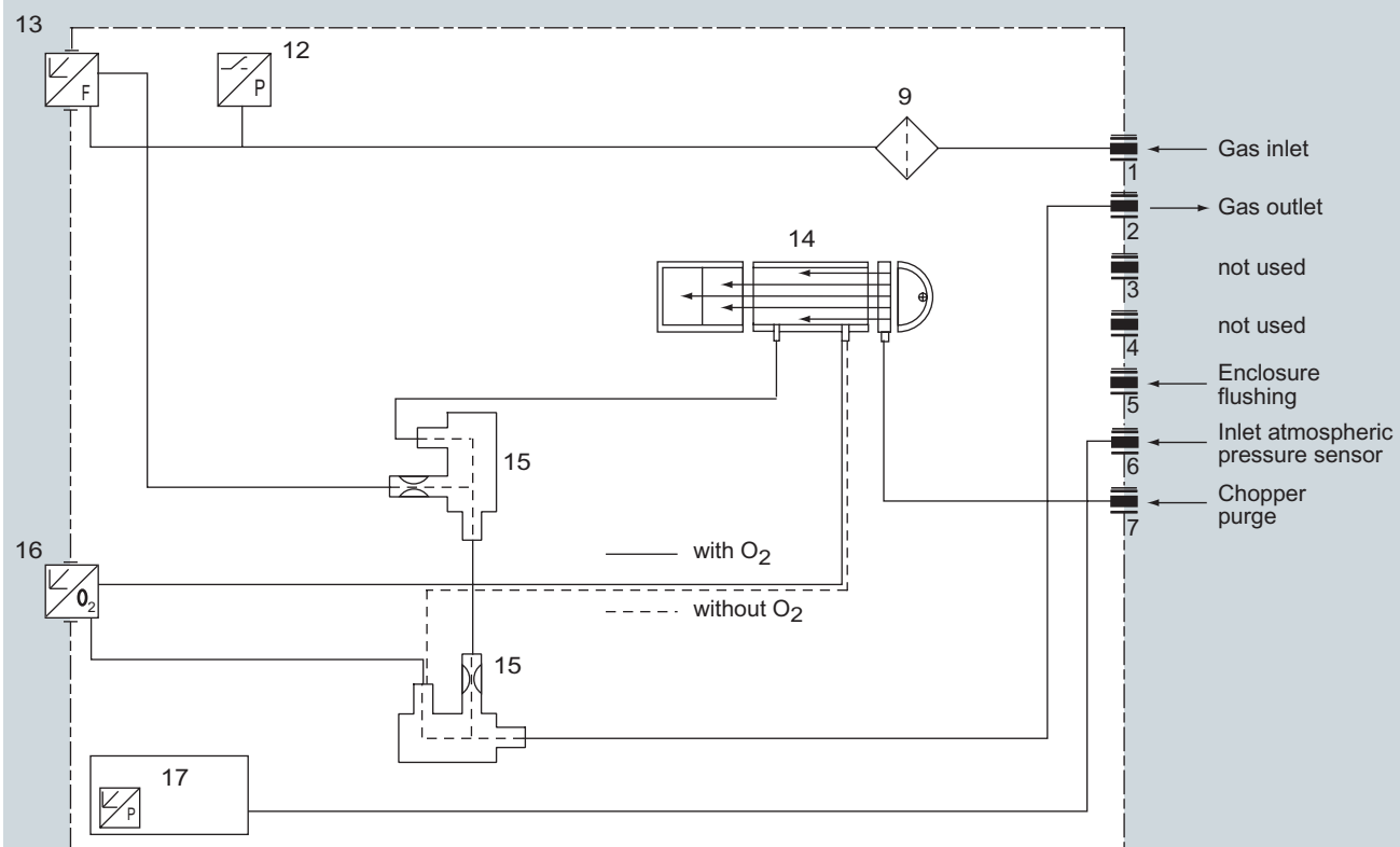
ULTRAMAT 23, 19" rack unit without internal sample gas pump, optional oxygen measurement
