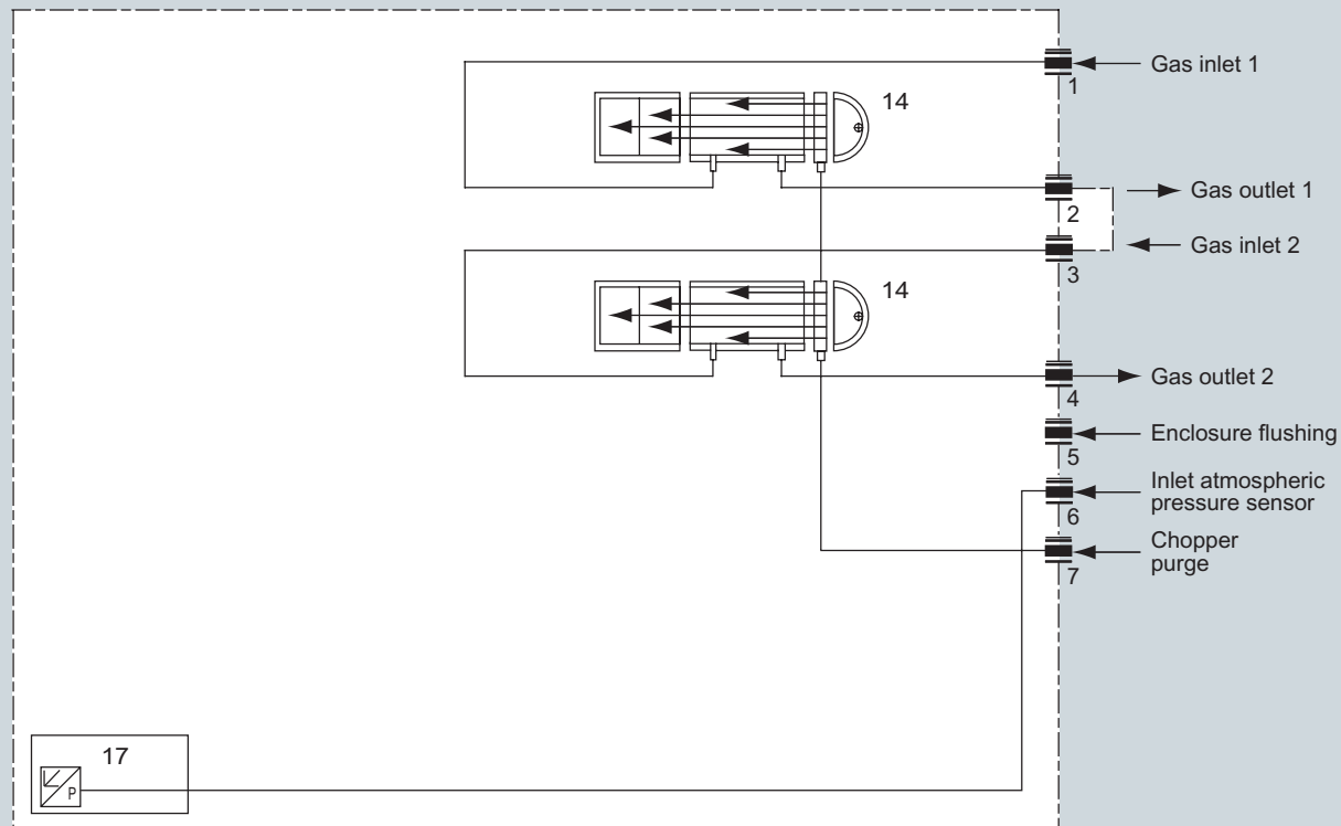
ULTRAMAT 23, 19" rack unit, sample gas path version in pipes, optional separate gas path, always without sample gas pump, without safety filter and without safety condensation trap
