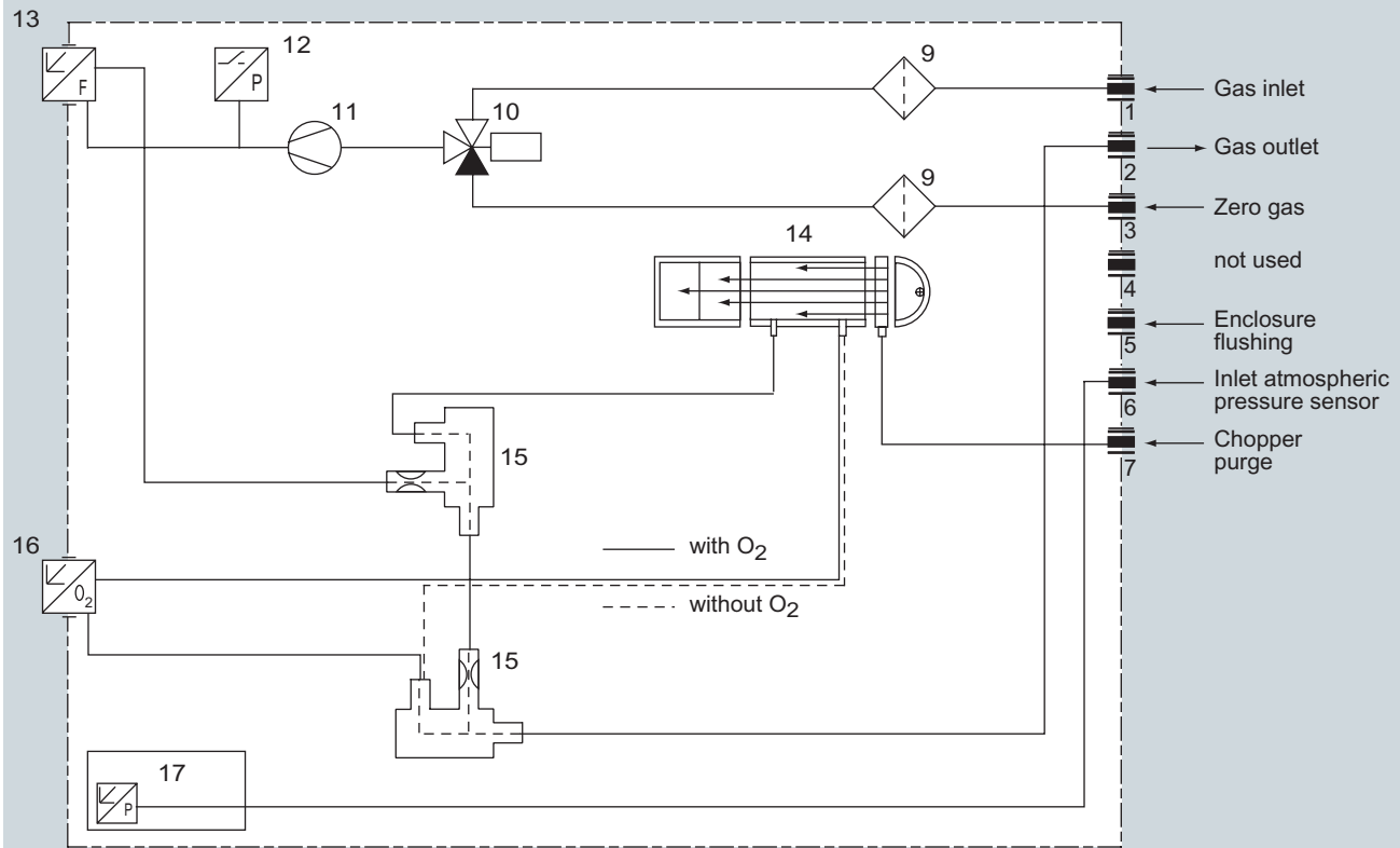
ULTRAMAT 23, 19" rack unit with internal sample gas pump, optional oxygen measurement
