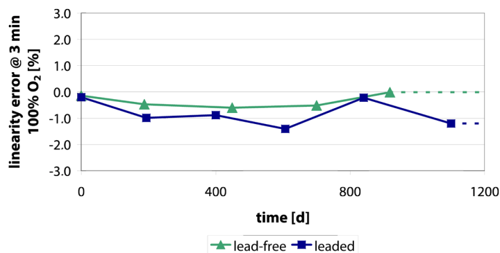
Linearity error
