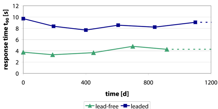
Response time t_{90}
