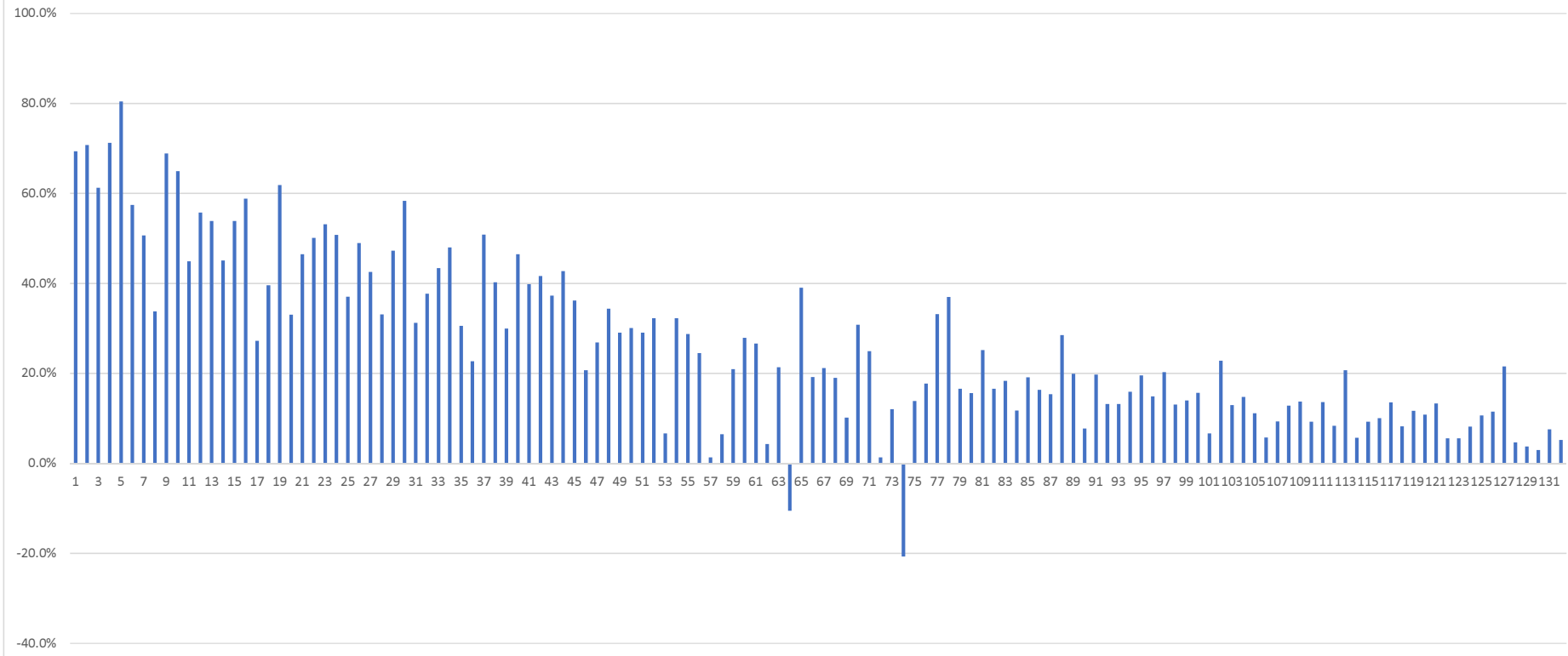
R-22A Percentage deviation for Returned Sensors '+7 Days' reading vs QA data (compensated for atmospheric pressure)
