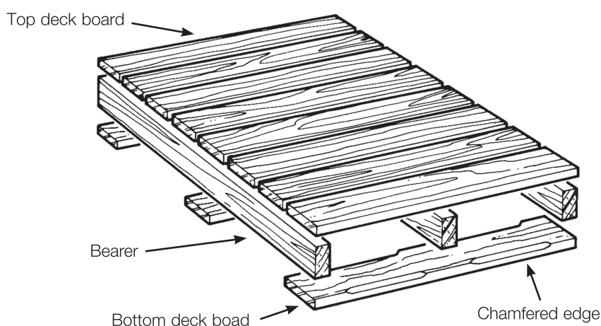
Figure 12(a) Four-way entry
