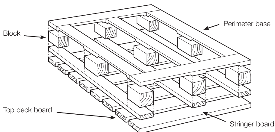
Figure 12(b) Four-way entry (underside view)
