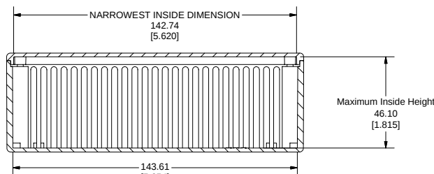
SECTION C-C
