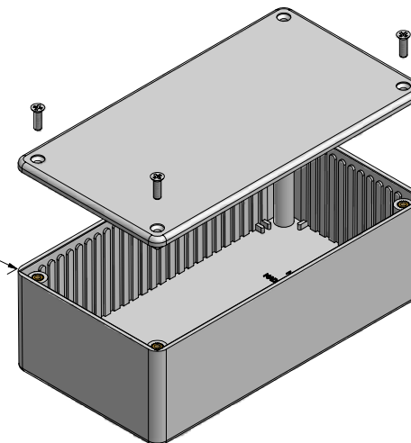
EXPLODED VIEW OF ENCLOSURE
