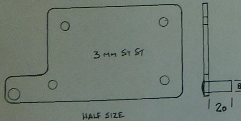
HINGE PIN PLATE 1 PAIR
