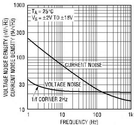
Noise Spectrum
