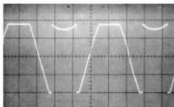
LM324, LM358, OP-20 EXHIBIT OUTPUT PHASE REVERSAL
