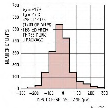
LT1014 Distribution of Offset Voltage
