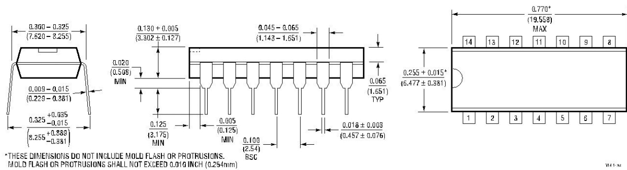
N Package 14-Lead PDIP (Narrow .300 Inch) (Reference LTC DWG # 05-08-1510)
