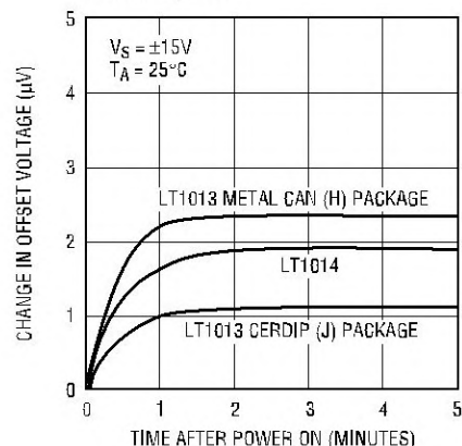
Warm-Up Drift
