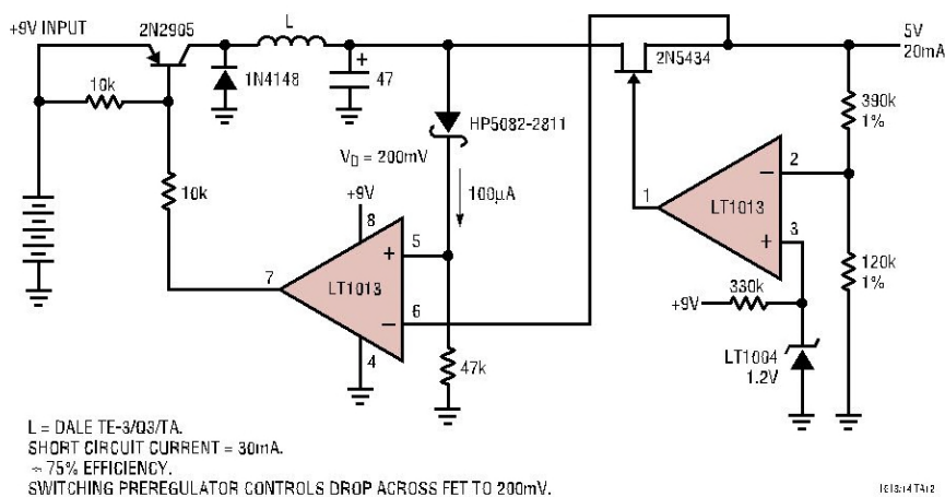
Low Power 9V to 5V Converter
