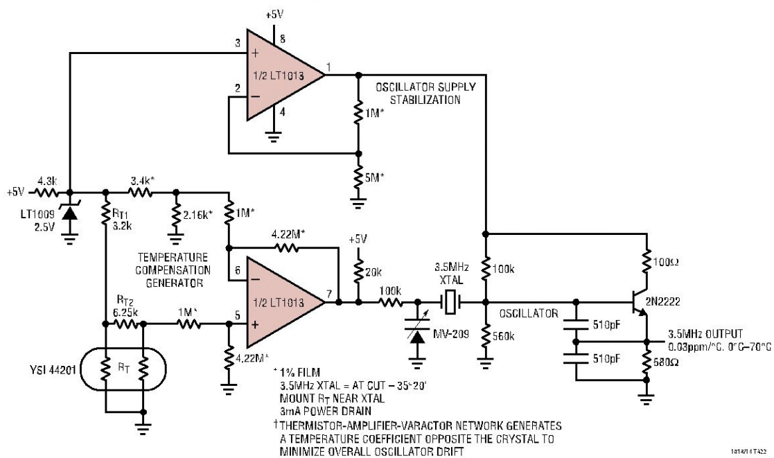
Low Power, 5V Driven, Temperature Compensated Crystal Oscillator (TXCO) †
