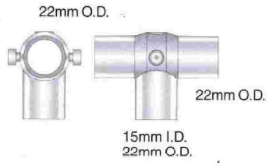
BE 125-1 Reusable tee adapter.
