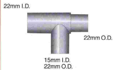
BE 117-W Disposable tee adapter. Blue
