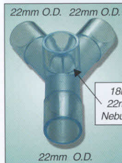
KC 211-D 60° Wye Connector
