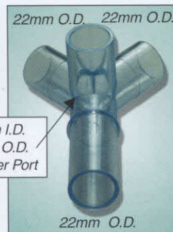
KC 212-D 90° Wye Connector
