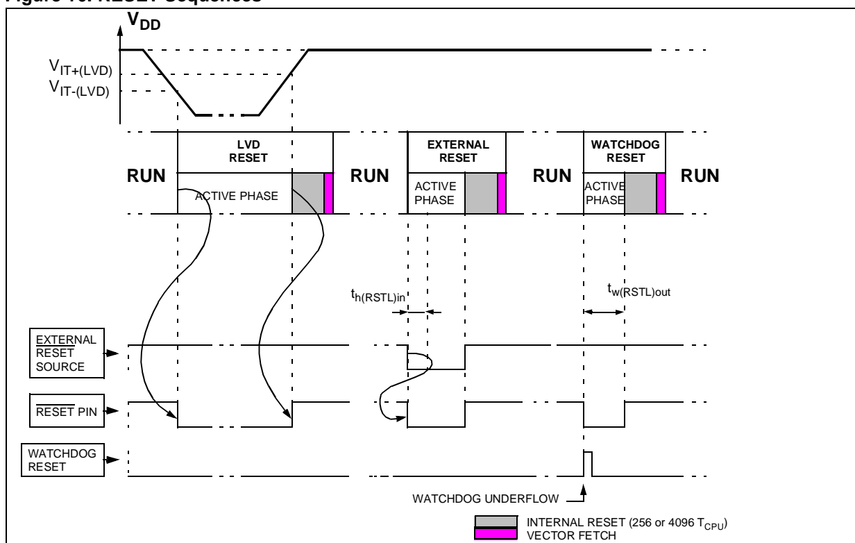
Figure 16. RESET Sequences
