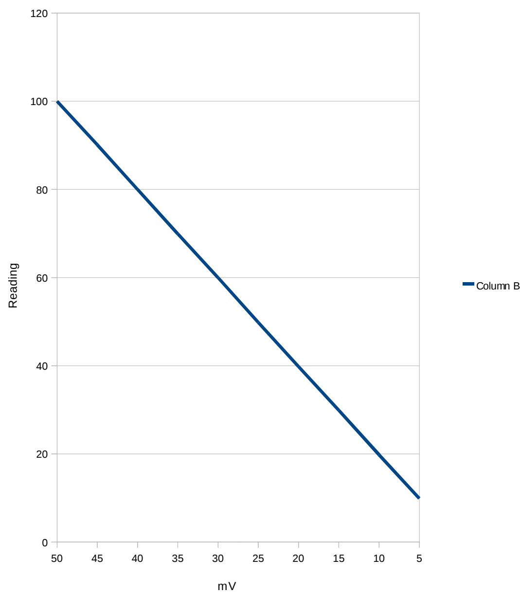
VN202 Lite Reading vs mV
