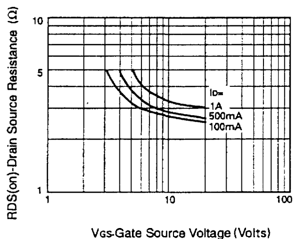
On-resistance v gate-source voltage
