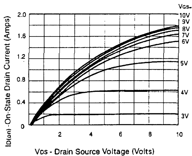
Saturation Characteristics
