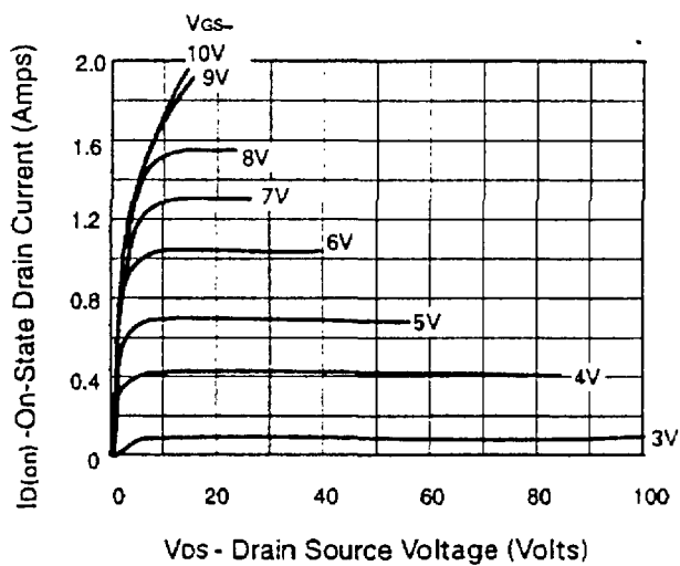
Output Characteristics
