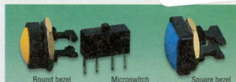
Round bezel: L = 23.1, Dia. = 19.8 Square bezel: L = 23.8, Bezel = 19.8 x 16
