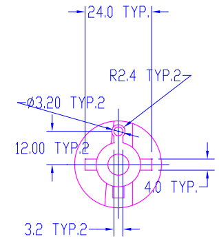
DETAIL P SCALE 2 : 1
