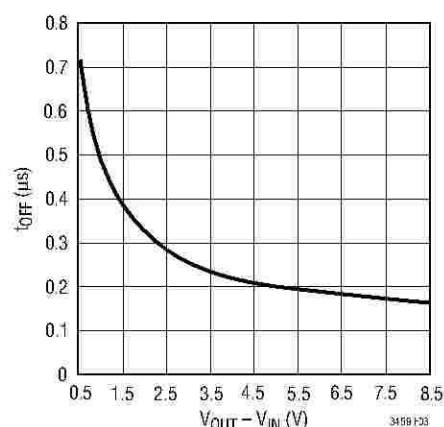
Figure 3. t_{OFF} Times
