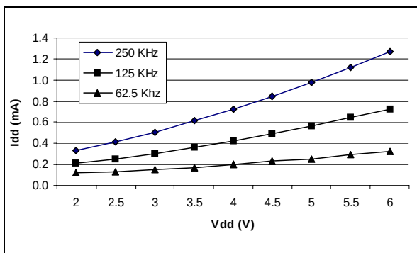
Figure 63. Typical I_{DD} in SLOW-WAIT vs. f_{CPU}
