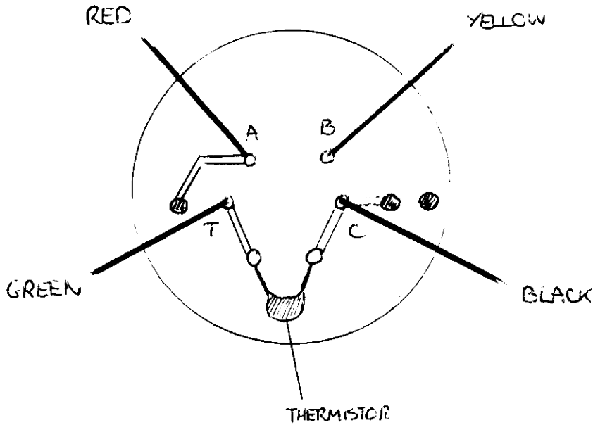
VIEW OF PCB IN SENSOR HOLDER FROM THE BACK (THE PINS WHICH CONTACT WITH THE CELL ARE ON THE OTHER SIDE OF PCB.)
