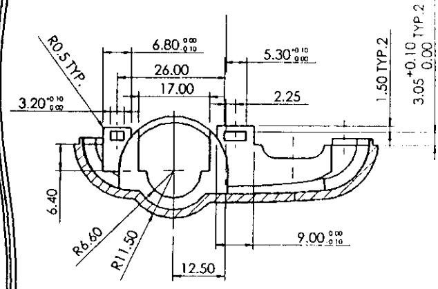
SECTION H-H
