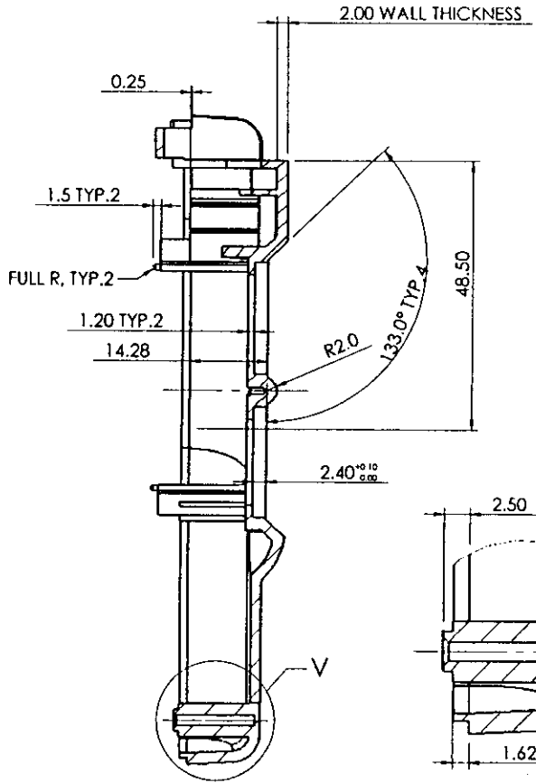
SECTION B-B
