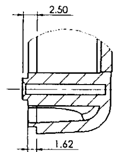
DETAIL V SCALE 1.5 : 1
