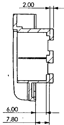
SECTION K-K
