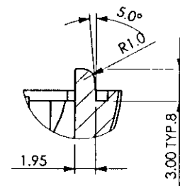
DETAIL V SCALE 2 : 1
