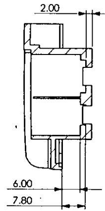
SECTION K-K
