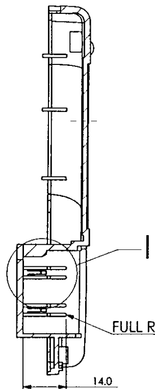
SECTION H-H
