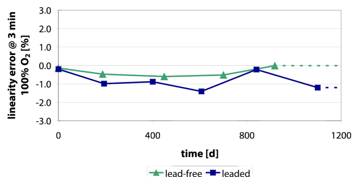
Linearity error
