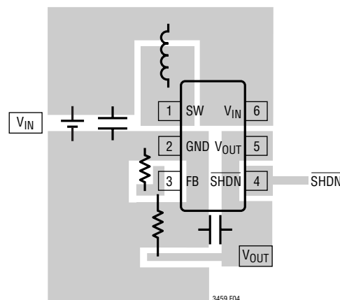
RECOMMENDED COMPONENT PLACEMENT. TRACES CARRYING CURRENT ARE DIRECT. TRACE AREA AT FB PIN IS SMALL. LEAD LENGTH TO BATTERY IS SHORT
