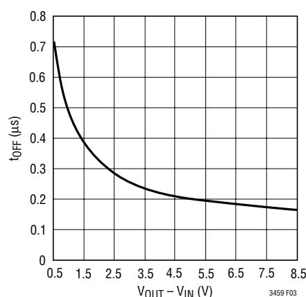
Figure 3. t_{OFF} Times
