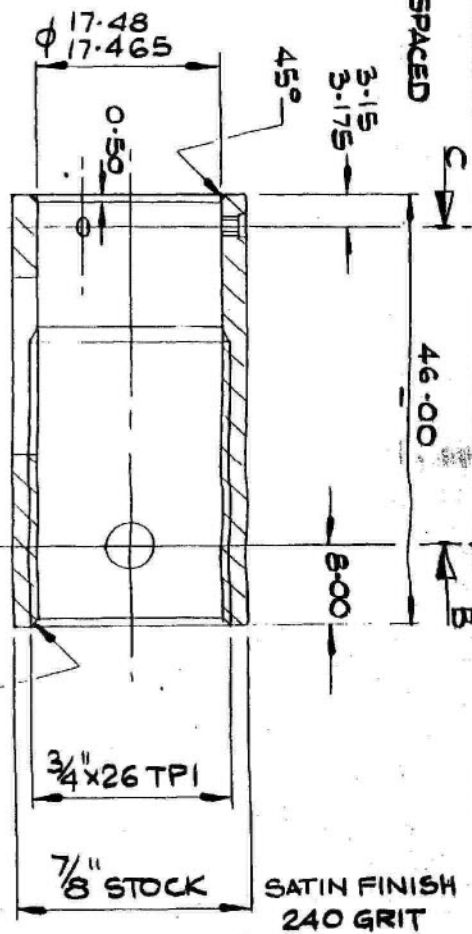
SECTION AA
