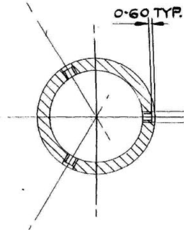
SECTION CC
