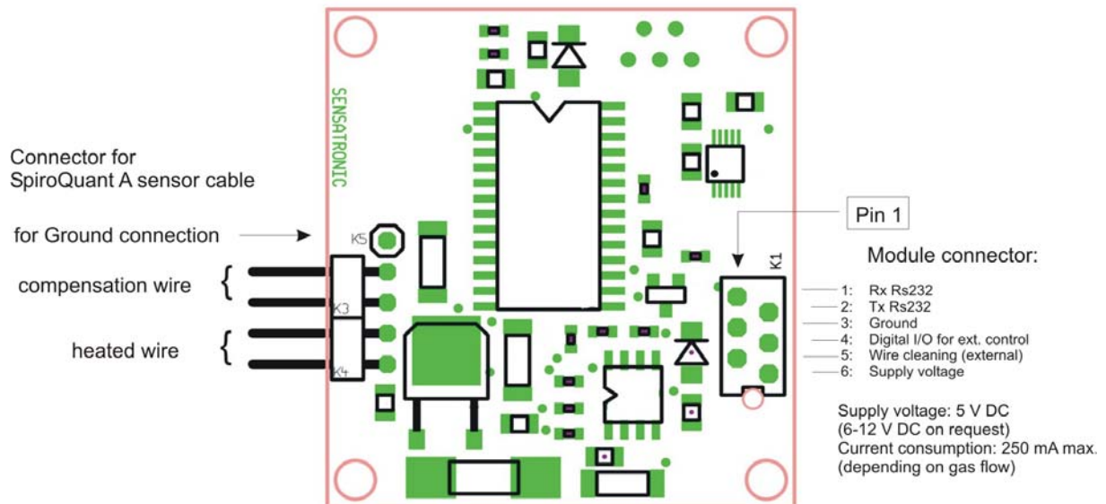
Figure 1: Main components of the PCB
