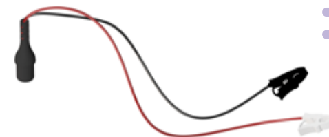
5750107 2510103 Stimulation Cable with pinch clamps* Overall length: 33.5 cm, each flying lead: 29.5 cm.
