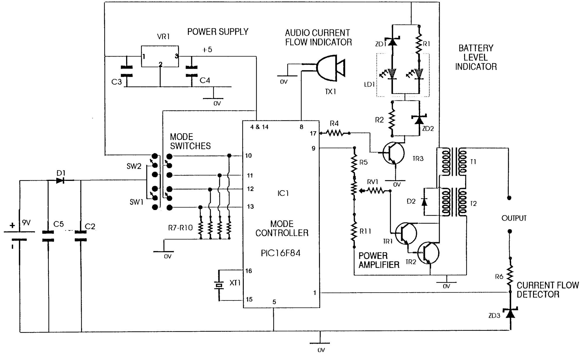
Microstim DB v2 Circuit diagram
