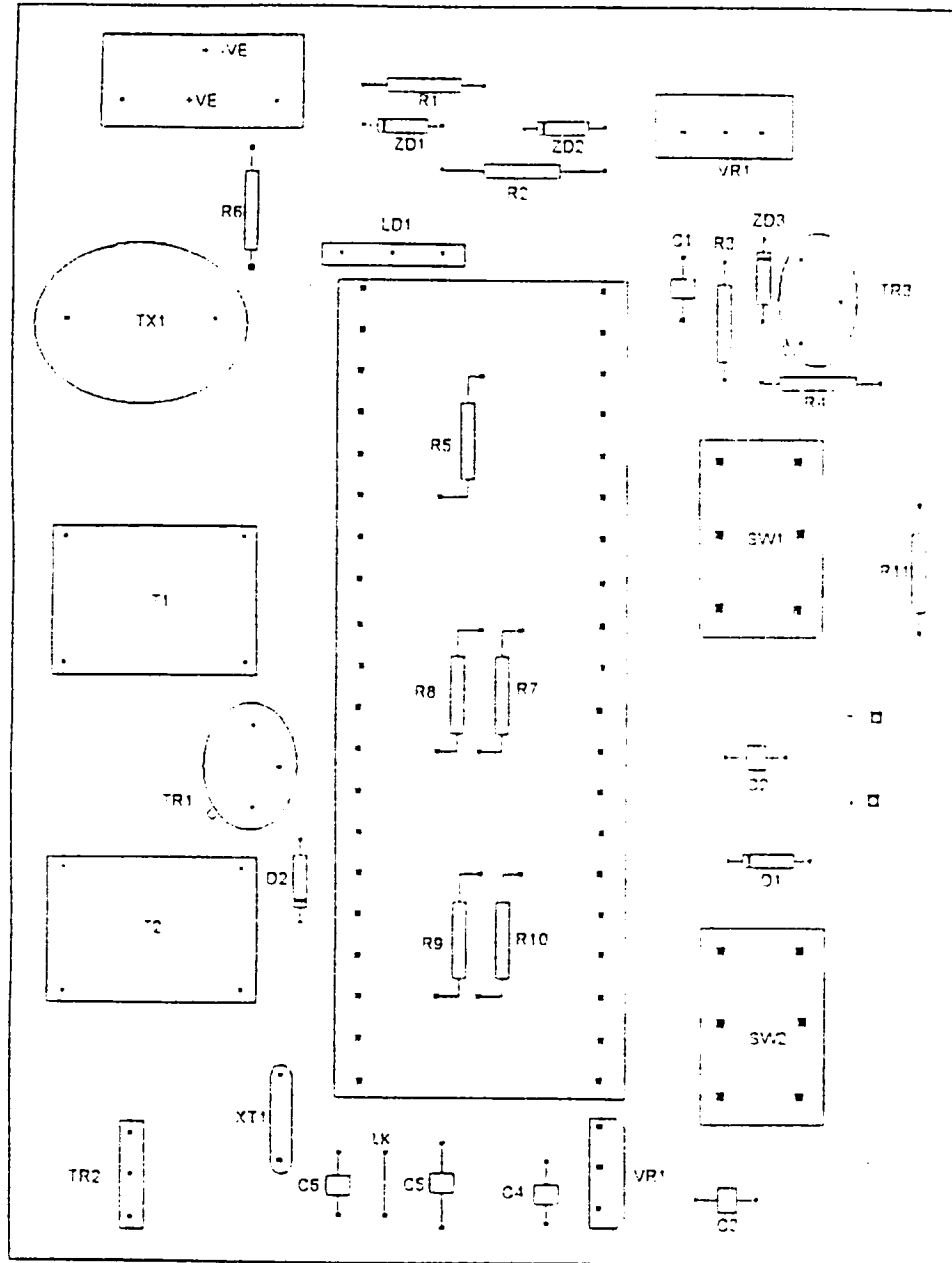
Microstim DB v1 Component layout
