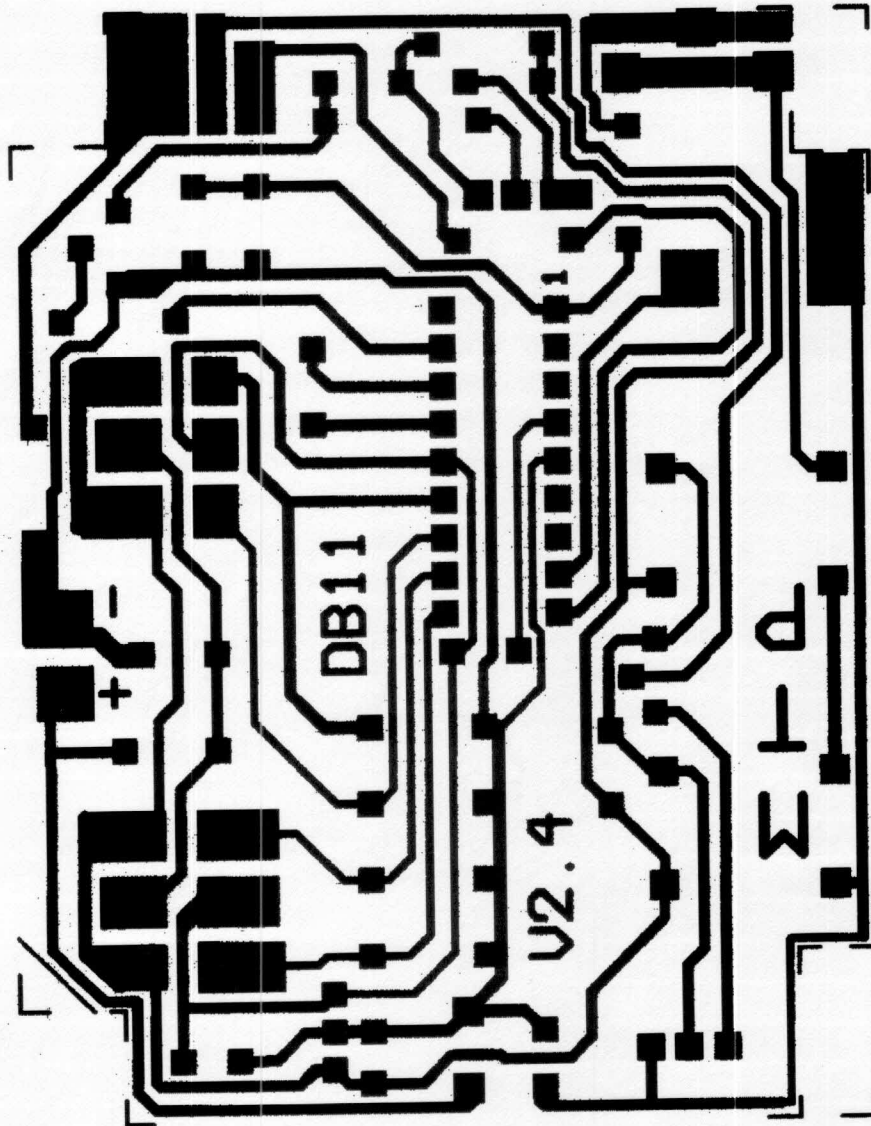
Microstim DB v2.4 PCB track layout
