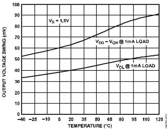
Figure 31. Output Voltage Swing vs. Temperature
