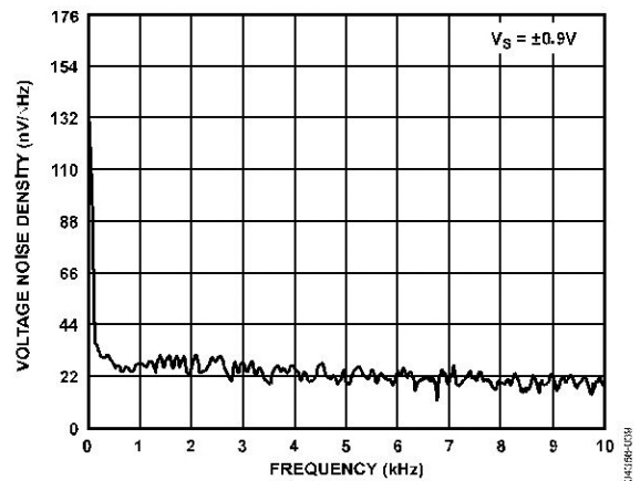
Figure 39. Voltage Noise Density vs. Frequency
