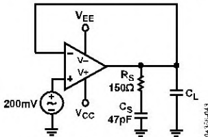
Figure 43. Snubber Network
