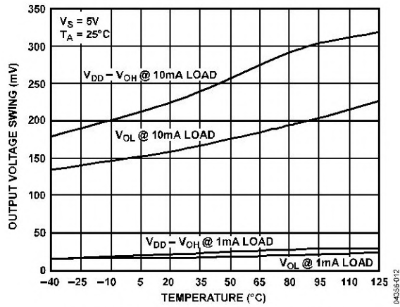
Figure 12. Output Voltage Swing vs. Temperature
