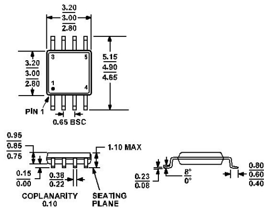
Figure 49. 8-Lead Mini Small Outline Package [MSOP] (RM-8)
