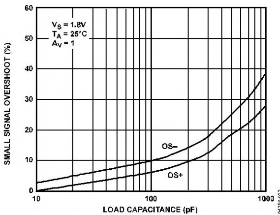
Figure 32. Small Signal Overshoot vs. Load Capacitance
