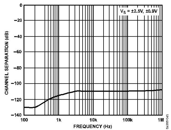
Figure 40. Channel Separation vs. Frequency
