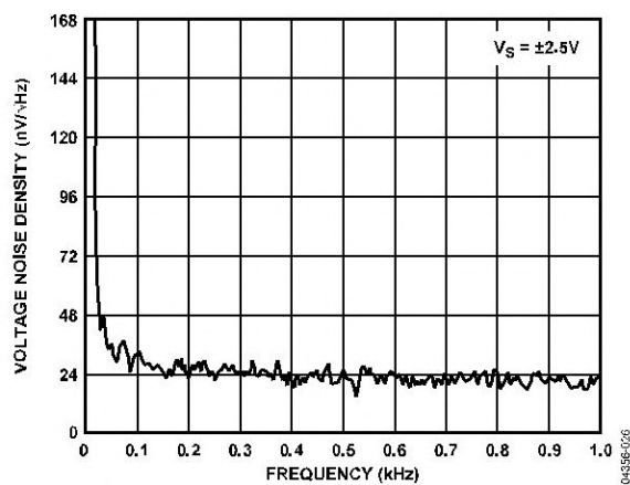
Figure 26. Voltage Noise Density vs. Frequency
