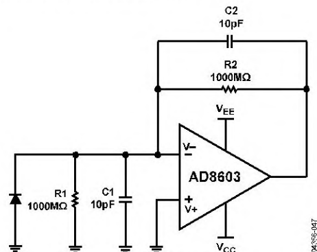
Figure 47. Photodiode Circuit
