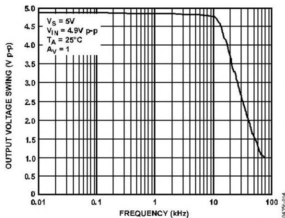
Figure 14. Closed-Loop Output Voltage Swing vs. Frequency
