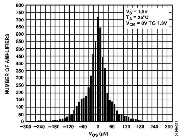
Figure 28. V_{OS} Distribution
