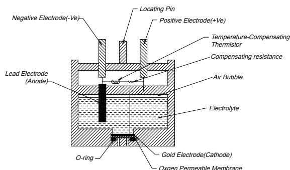
Fig. 1 - Structure of SK-25F
