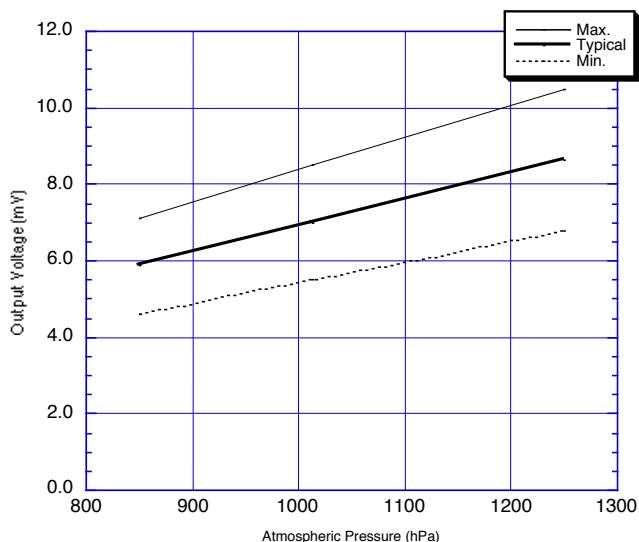
Fig. 5 - SK-25F response of output voltage to ambient pressure changes (at 25°C/60%RH)
