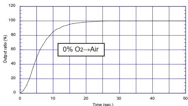
Fig. 4 - Response speed of SK-25F to oxygen
