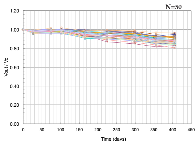
Fig. 10 - SK-25F long term stability
