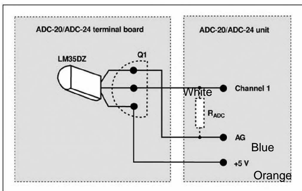
Temperature sensor circuit with LM35 IC
