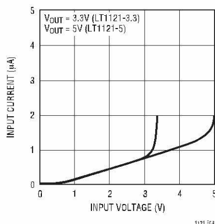
Figure 3. Input Current
