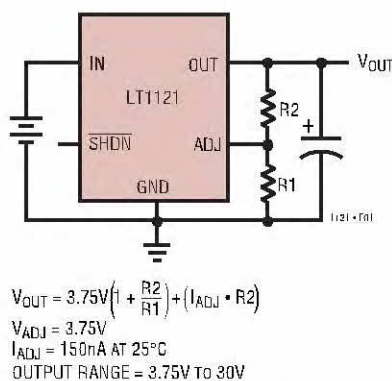
Figure 1. Adjustable Operation
