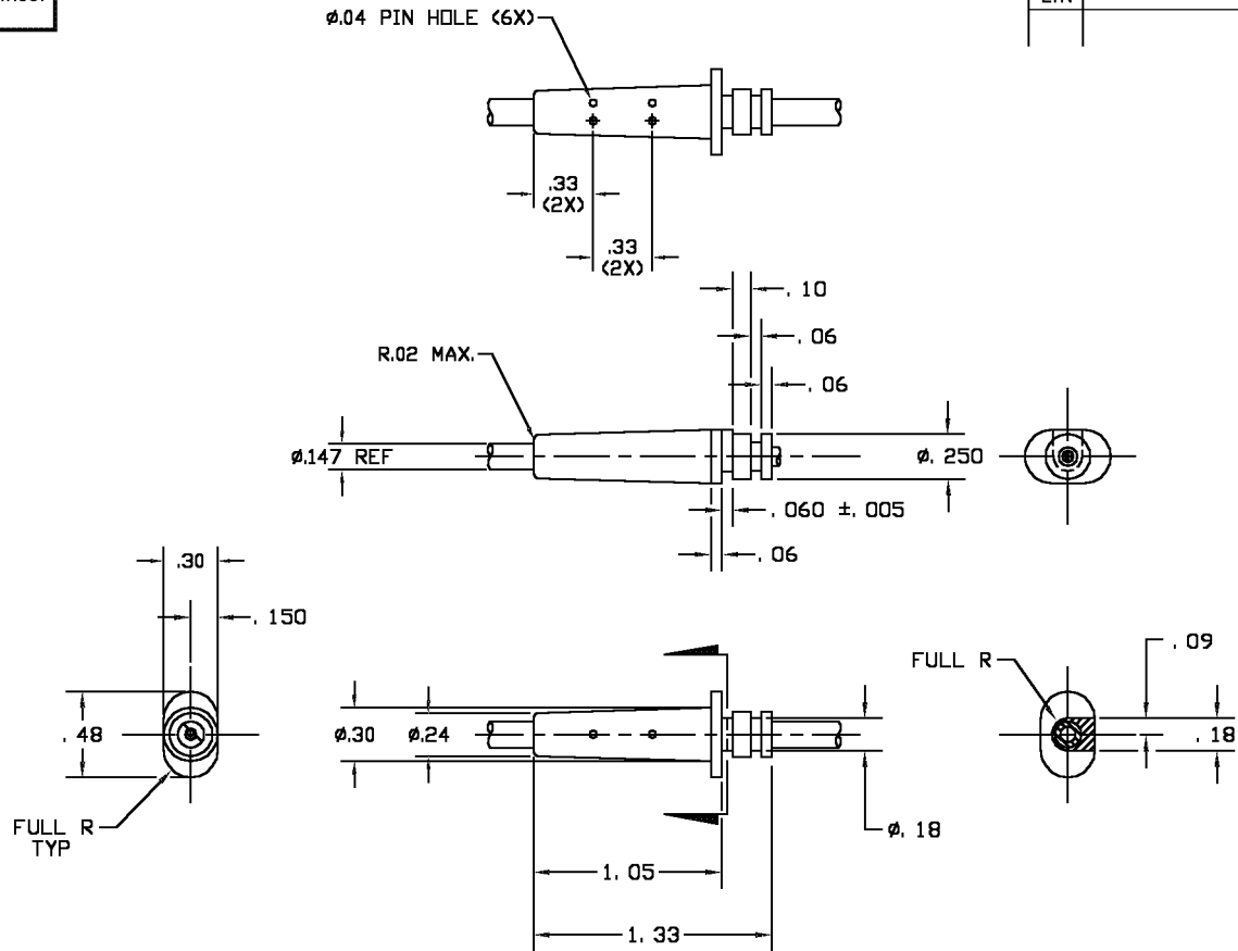
DETAIL B
