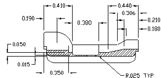
Section View BB
