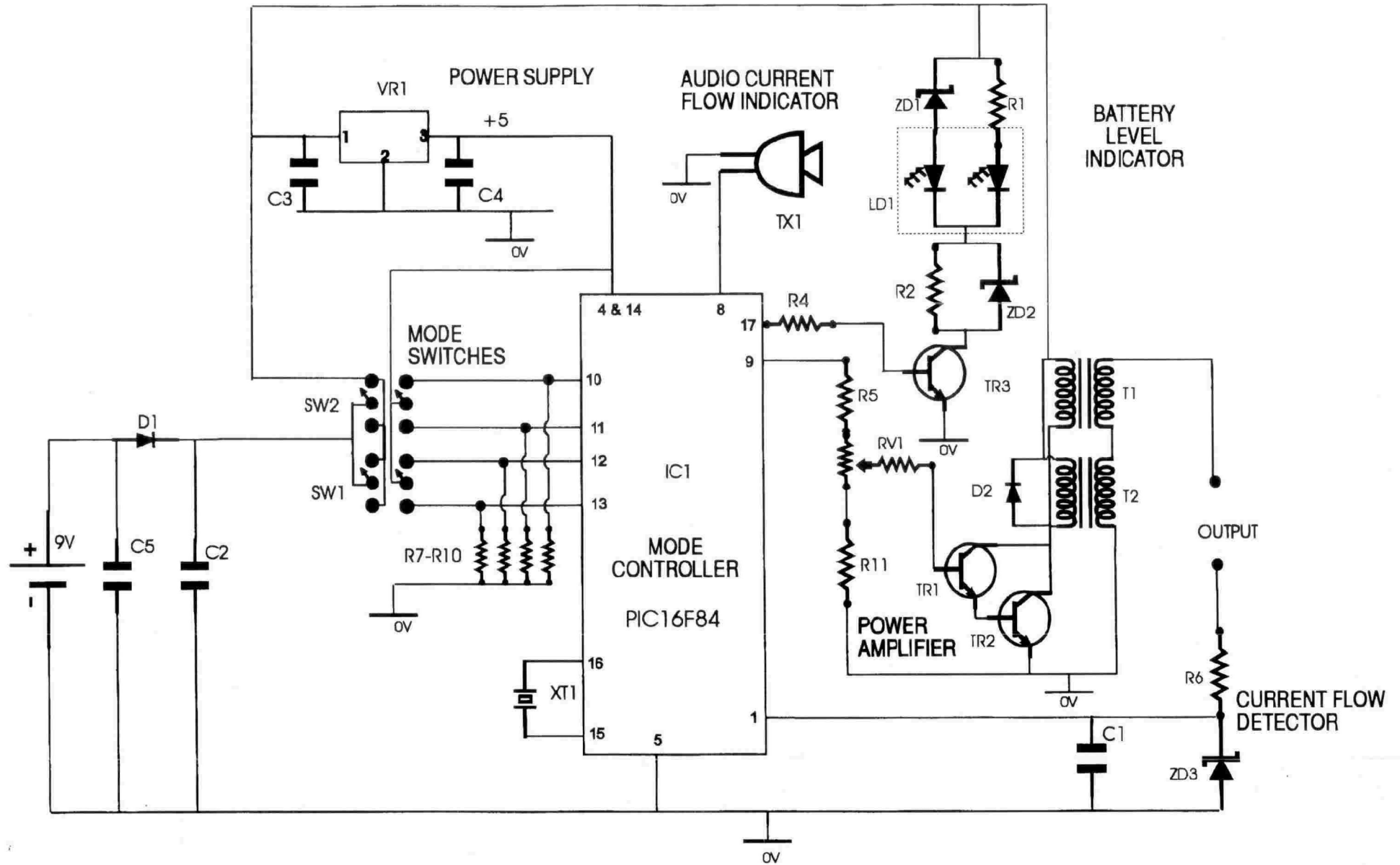
Microstim DB v2.4 Circuit diagram
