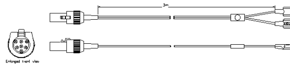
Hypertronics male 7 pin
