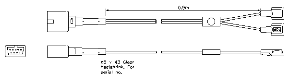
D-Type Male 9 Pin
