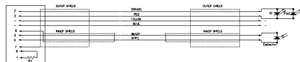
D-type male 9 pin
